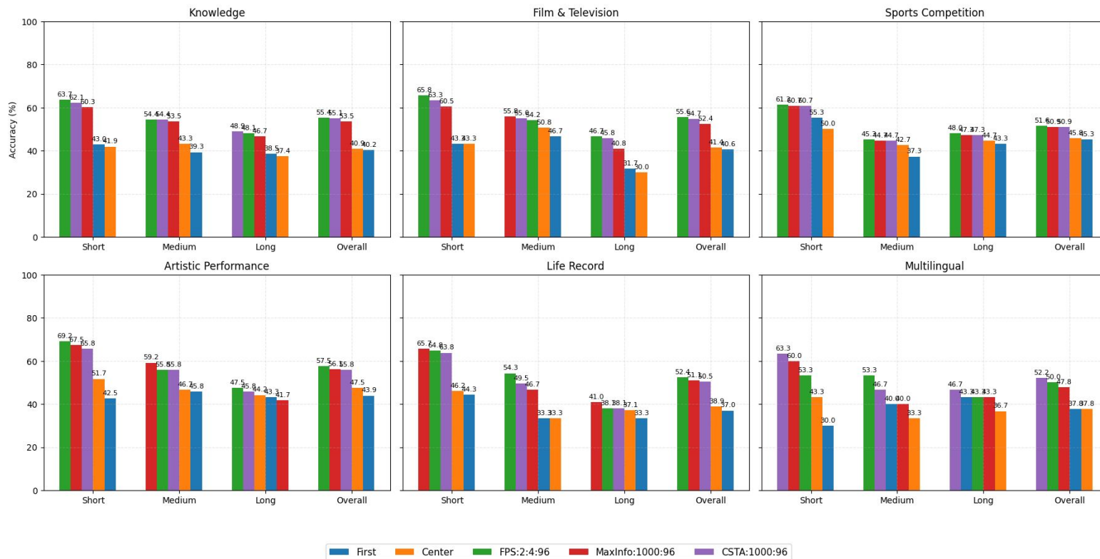
Ovis2 performance on VideoMME for Video Categories and Sampling Techniques
