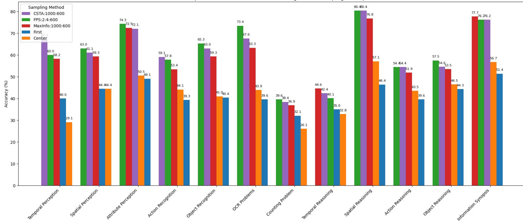
Qwen2.5 performance on VideoMME for Taks Categories and Sampling Techniques
