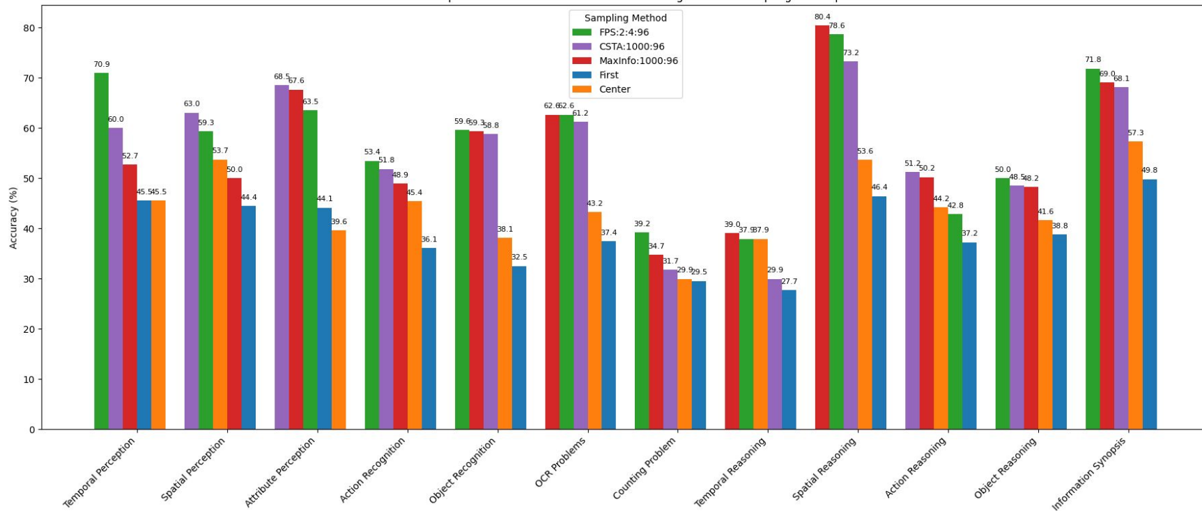
InternVL3 performance on VideoMME for Taks Categories and Sampling Techniques
