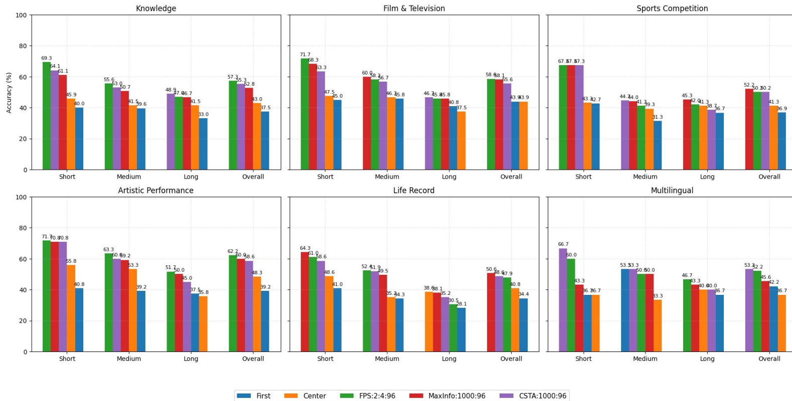
InternVL3 performance on VideoMME for Video Categories and Sampling Techniques
